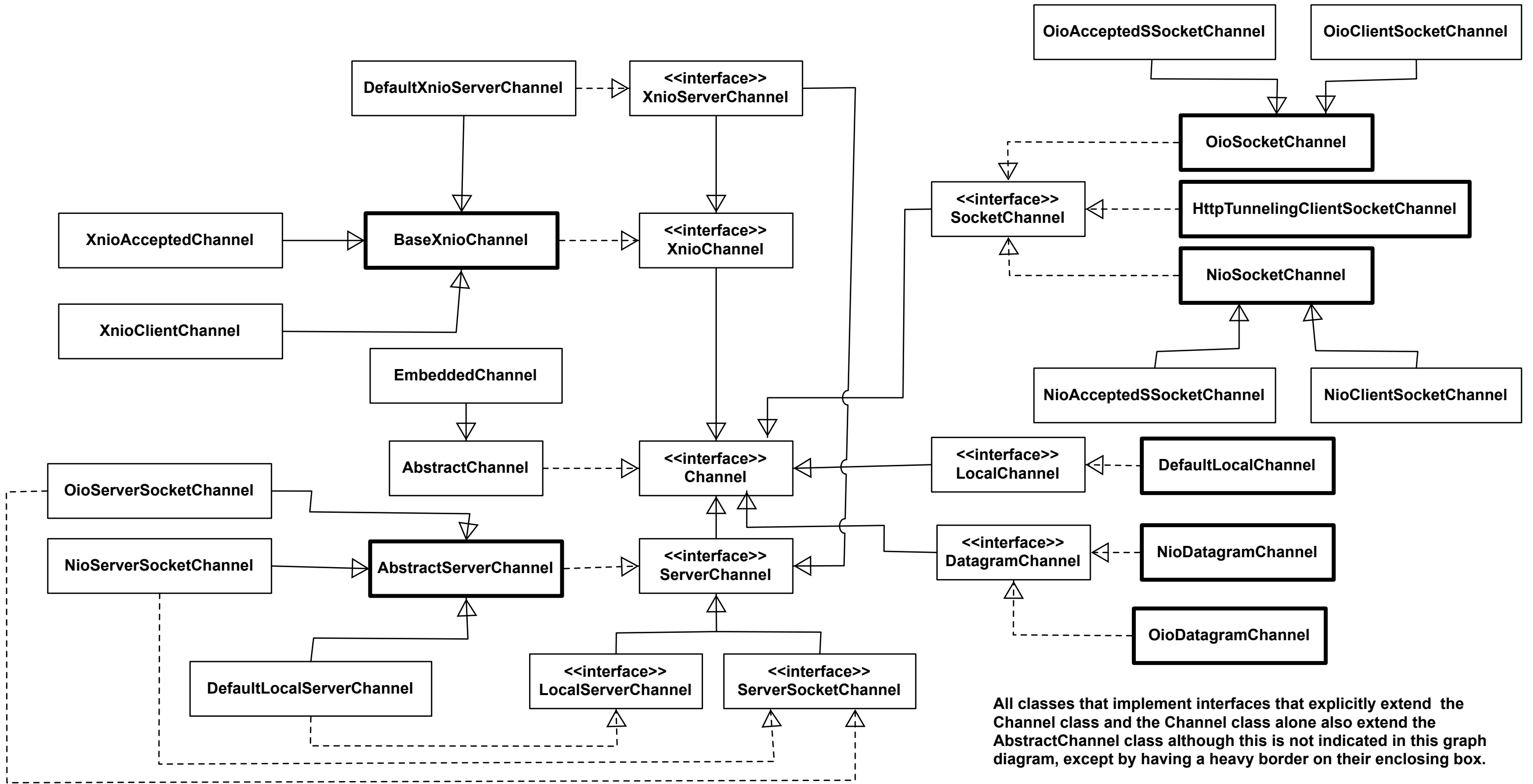
Diagram of the Netty Channel Class Extended Graph
