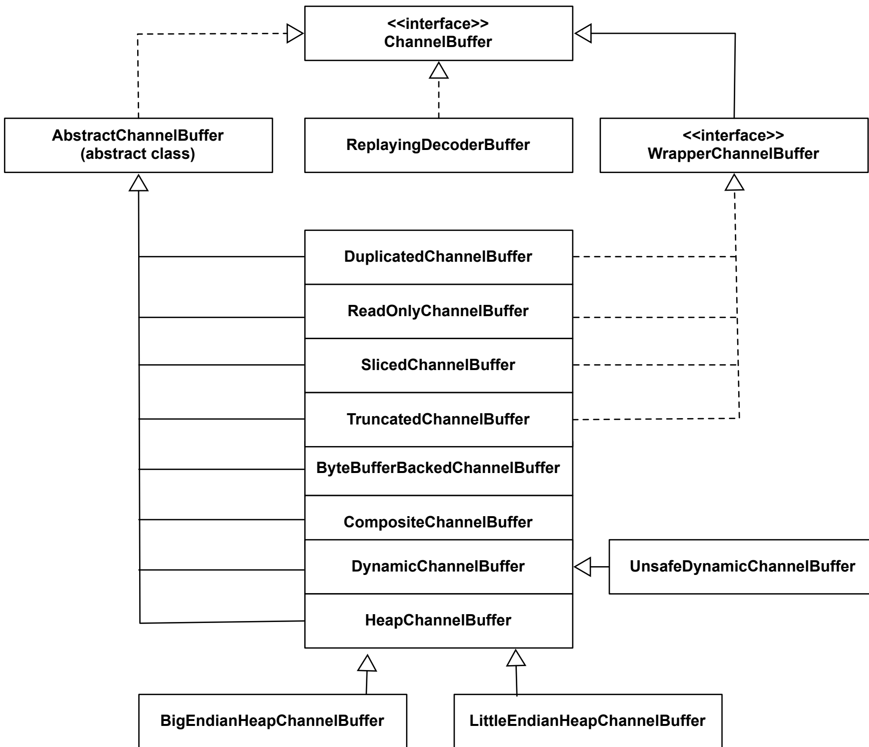
Diagram of the Netty ChannelBuffer Class Extended Graph
