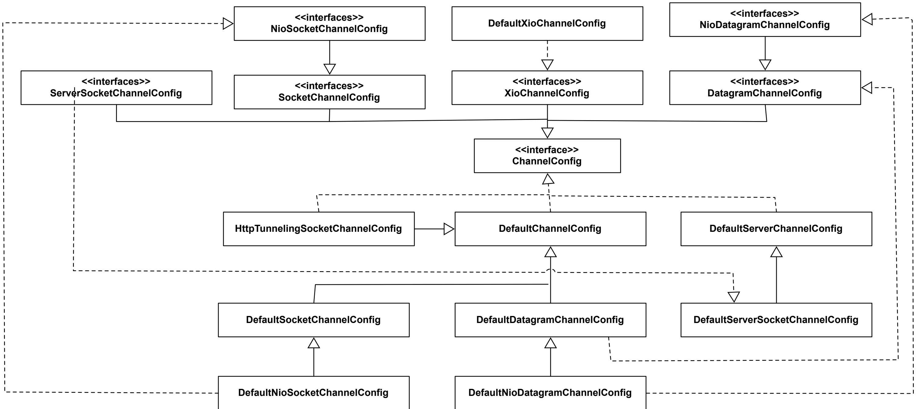
Diagram of the Netty ChannelConfig Class Extended Graph
